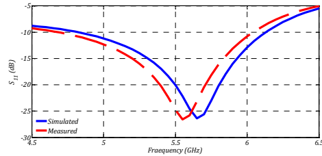
Figure 2. the simulated and measured return loss of the proposed antenna
