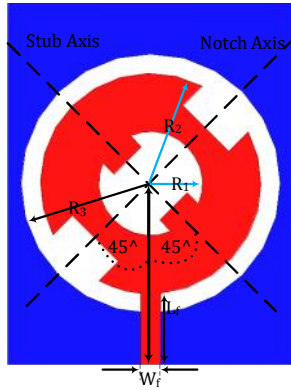
Figure 1 Antenna configurations.
