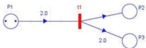
Figure 1. A simple Petri Net
