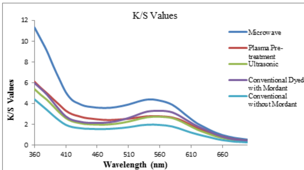
Figure 2. The K/S values of the dyed silk samples
