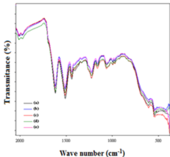
Figure 4. FT-IR ATR spectra: (a) conventional dyeing without mordant; (b) silk fabric with plasma treatment; (c) conventional method with mordant; (d) microwave method; (e) ultrasonic method
