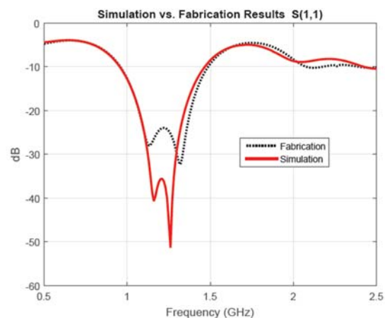
Figure 5. Measured and simulated diagrams of S11 parameter for proposed antenna (Ant.5).
