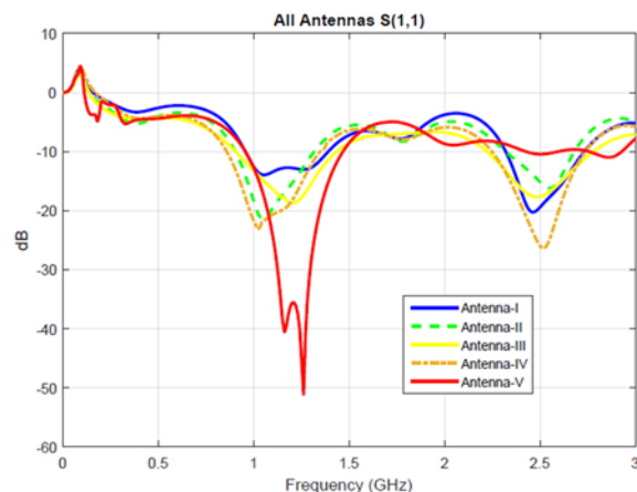
Figure 4. S11 graphs of simulated antenna.
