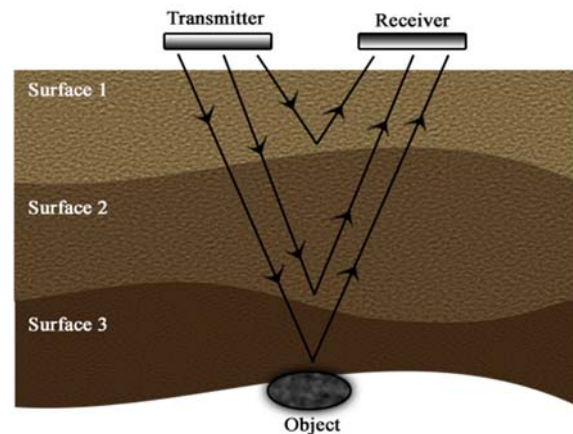
Figure 1. General working principle of GPR.
