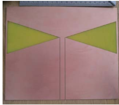
Figure 7. Photograph of fabricated Bow tie Antenna
