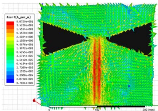
Figure 6. Current distribution demonstration.
