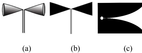
Figure 2. Some GPR antennas; (a) Biconic antenna, (b) Bow-tie antenna, (c) Vivaldi antenna.
