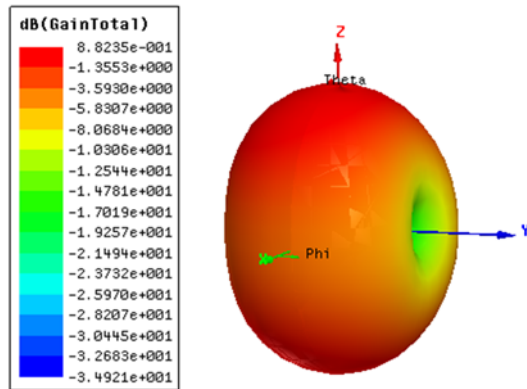
Figure 9. 3D antenna gain plot.
