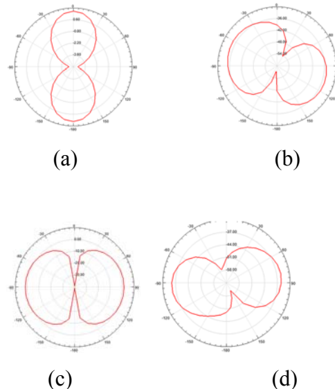
Figure 8. Radiation pattern of proposed antenna at (a) \phi=0^\circ , (b) \phi=90^\circ , (c) \theta=0^\circ and (d) \theta=90^\circ .
