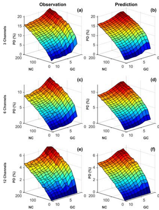
Figure 3. Observations and corresponding predictions for various channels (NC: Node count, GC: Gateway count, PD: Packets dropped).
