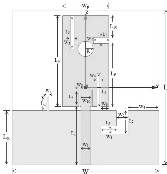
Figure 4. Complete Design Parameters of Antenna
