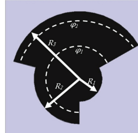
Fig. 2. Configuration of proposed fractal
