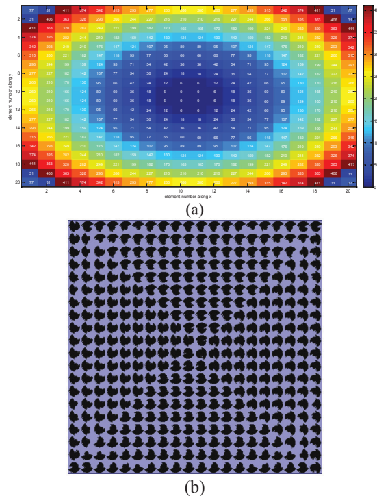
Fig. 4. The mask of the reflectarray antenna and the obtained reflection phase of the elements
