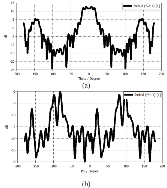
Fig. 5. Pattern of proposed antenna at 4.4GHz (a)co-polarization (b)cross polarization
