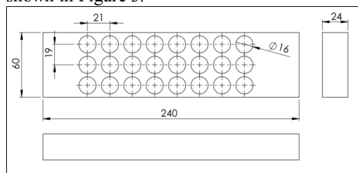
Figure 3. Experimental specimen
