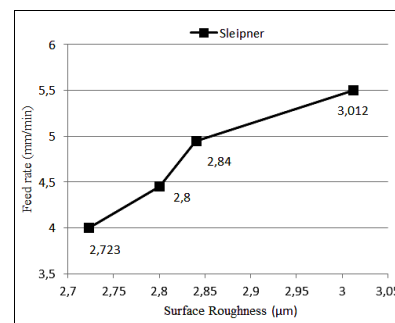
Figure 6. The effect of surface roughness against feed rate (IP : 35,1A – On time: 15,3 \mu s - V:40V - Off time:17 \mu s - CP: 5kg/cm 2 - VW: 12m/min - WD: 0,3mm - WT: 9kg)
