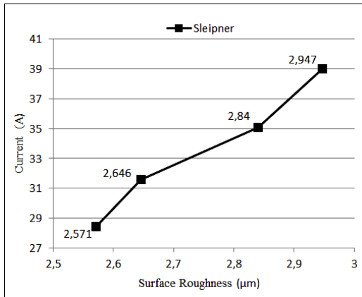
Figure 7. The effect of surface roughness against current value (SF:4,95mm/min – On time: 15,3μs - V:40V - Off time:17μs - CP: 5kg/cm2 - VW: 12m/min - WD: 0,3mm - WT: 9kg)
