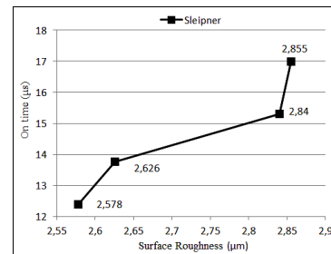
Figure 5. Effect of surface roughness against on time duration (IP : 35,1A - SF:4,95mm/min - V:40V - Off time:17 \mu s - CP: 5kg/cm 2 - VW: 12m/min - WD: 0,3mm - WT: 9kg) Proportional increase in surface roughness with the increase of on time duration in Figure 5 is shown. Although a 10% increase the variable parameter the on time duration, the first 1%, the other is the increase in the amount increased by 8% and 5% on results. Increase the size of the crater of on time duration increases, so also means increasing roughness. Graphics also defends this thesis.
