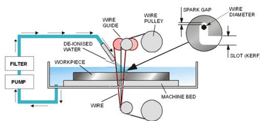
Figure 2. Schematic of wire erosion process [10]
